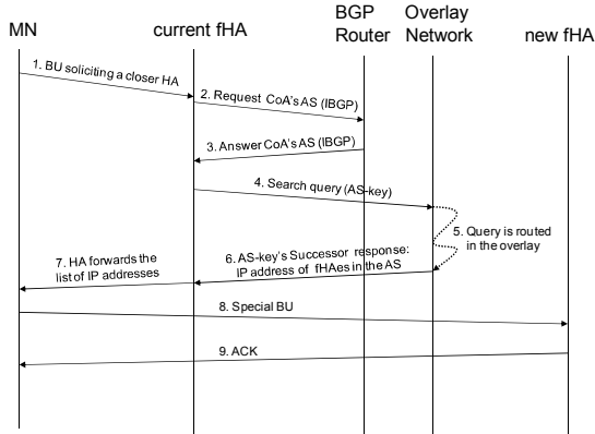
Figure 2. fHA Discovery Phase in the fP2P-HN architecture
