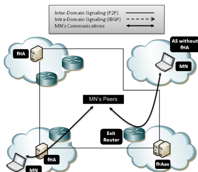
Figure 1. Overview of the fP2P-HN architecture
