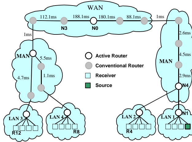
Fig. 2. Simulated topology
