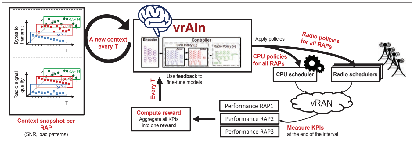
Figure 5. AI-based closed control-loop vRAN resources management for slicing [12].
