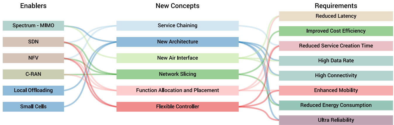
FIGURE 1 Fifth-generation (5G) new concepts, enablers, and requirements. The figure identifies the enablers upon which each concept relies and which requirements it contributes to satisfy. C-RAN, centralized radio access network; MIMO, multiple-input multiple-output; NFV, network function virtualization; SDN, software-defined networking
