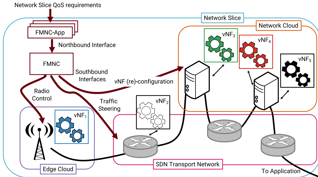
FIGURE 4 An example of the flexible mobile network controller (FMNC). QoS, quality of service; VNF, virtual network function
