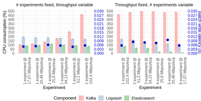
Fig. 4. CPU consumption and batch write latency evolution for 100 B data traffic in different experiments, modifying a different design parameter in each case whereas the other one remains fixed.
