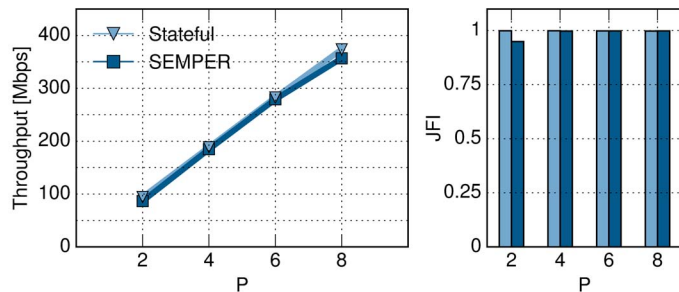
Fig. 4: Performance evaluation in static scenarios, N = 4 hosts
