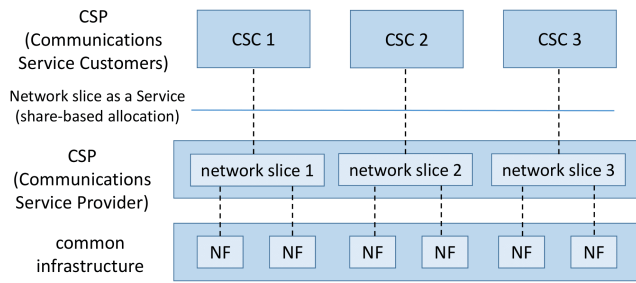
FIGURE 2: 3GPP management of share-based models.
