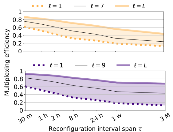
FIGURE 4: Efficiency of the reservation-based approach versus the resource reconfiguration periodicity \tau . Dashed and solid colored lines denote the \ell = 1 (edge resources) and \ell = L (central resources), while the black solid line follows an intermediate network level. Top: Large metropolis. Bottom: medium-sized city. Source: [23].
