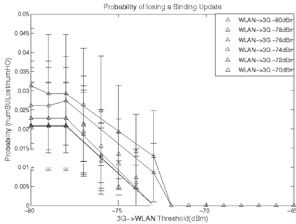
Figure 6: Probability of losing a Binding Update for several thresholds
