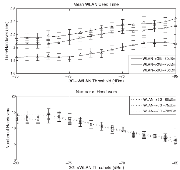
Figure 5: Wireless LAN Time usage and number of handovers
