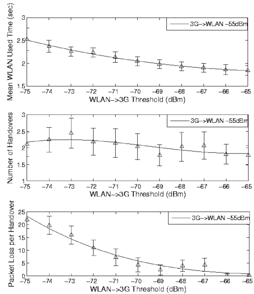
Figure 9: Study of the performance obtained for 0 packet loss
