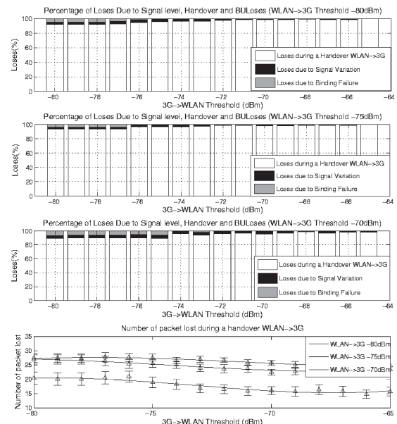
Figure 8: Study of the different contributions to the packet loss
