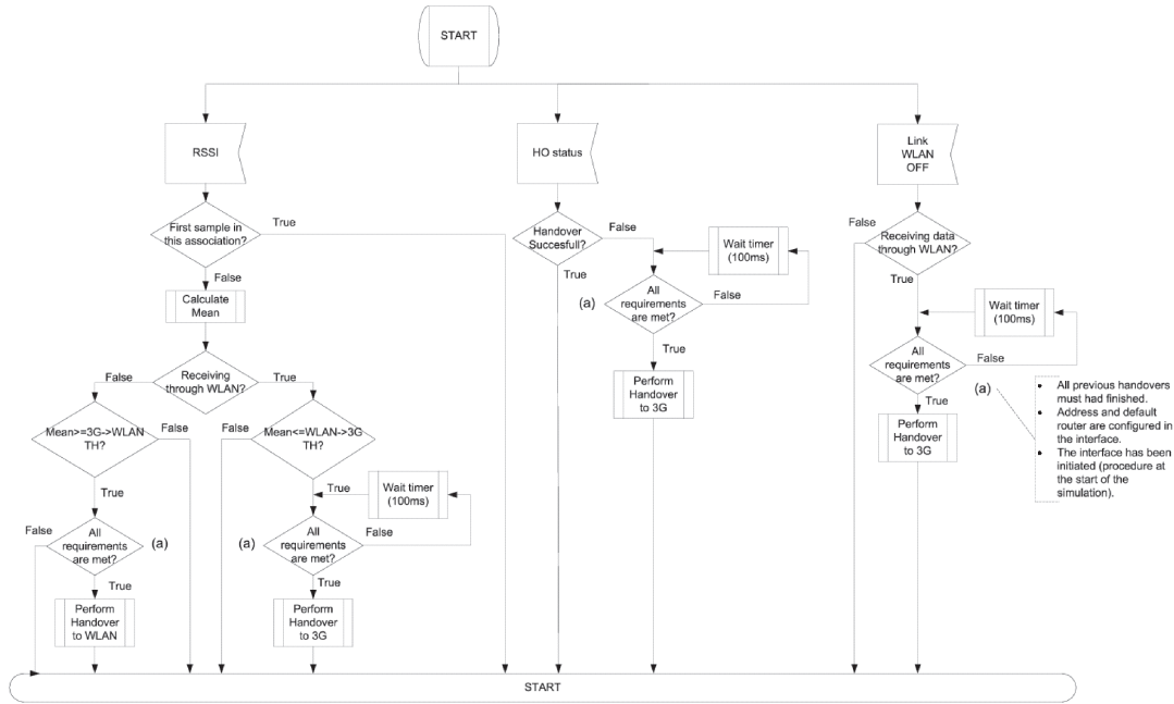
Figure 3: Handover Algorithm Flow Diagram
