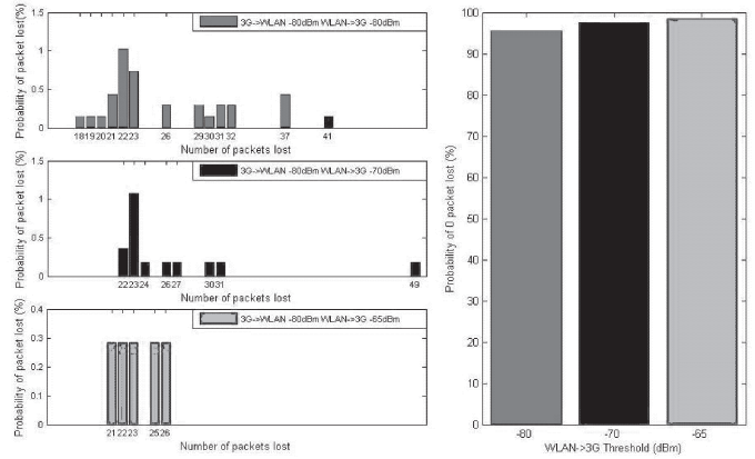
Figure 7: Effect of the thresholds in the packet loss due to variation of the signal level
