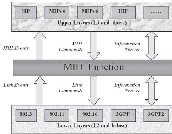
Figure 1: IEEE 802.21 MIH reference model
