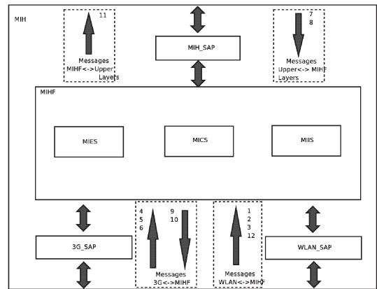
Figure 2: IEEE 802.21 MIH OMNET++ model
