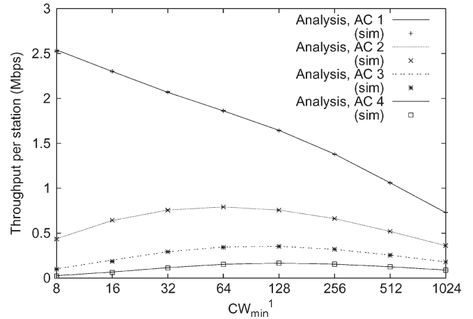
Fig. 5. Validation of the throughput model for a scenario with four ACs, each using a different AIFS and CW configuration.
