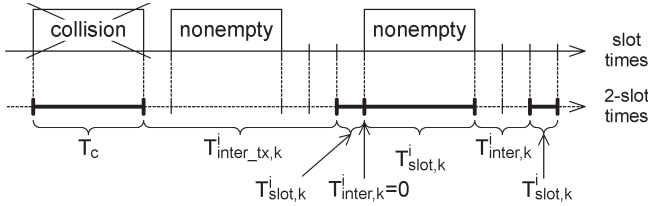
Fig. 4. Components of the delay (example with k = 2 ).
