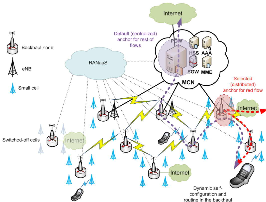
Figure 3 Distributed mobility management solution
