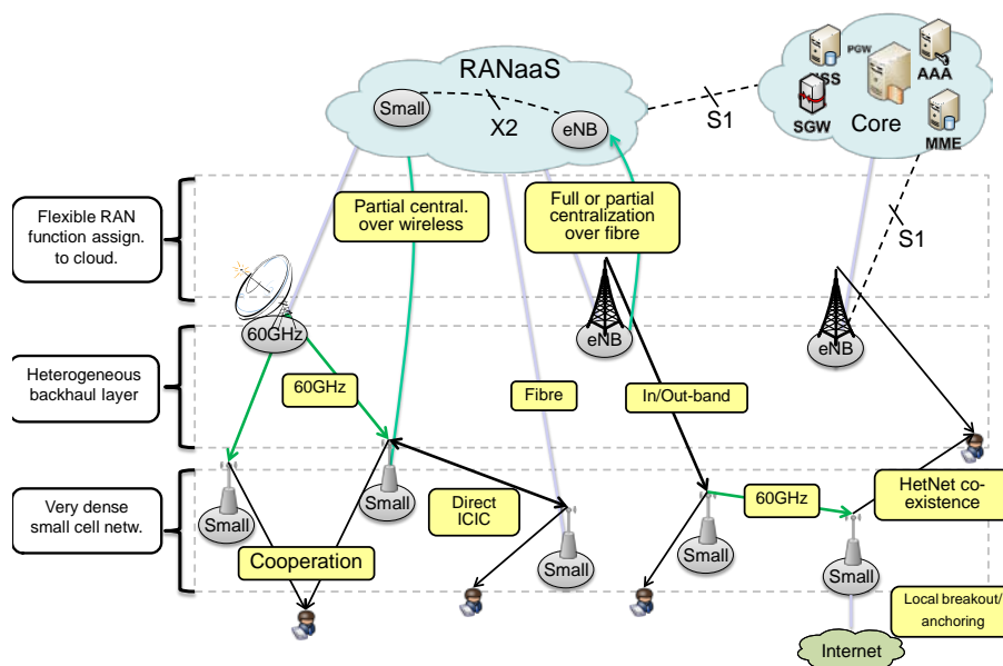
Figure 1 Considered mobile network architecture
