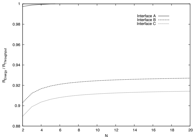
Fig. 10. Relative throughput loss for the energy-optimized configuration
