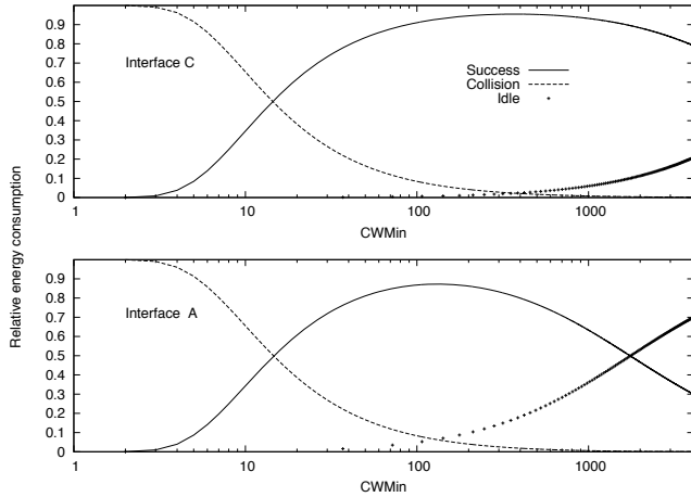
Fig. 3. Relative energy devoted to collisions and idling for the selected energy profiles A and C from Table I
