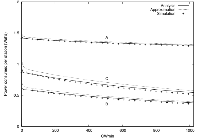
Fig. 2. Power consumption for the energy profiles of Table I for different CW_{min} configurations, N = 10 .
