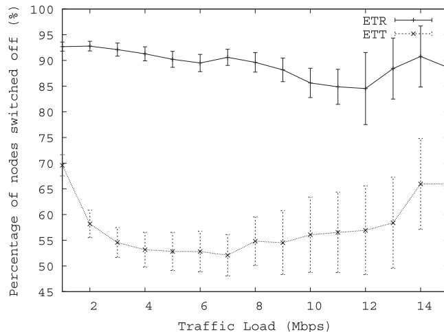
Fig. 16. Energy savings vs. ETT, 10 GW/Source nodes.
