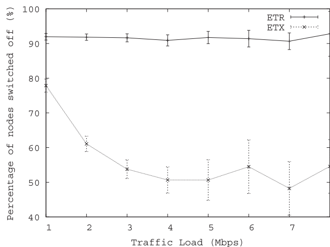
Fig. 17. Energy savings vs. ETX, 10 GW/Source nodes.
