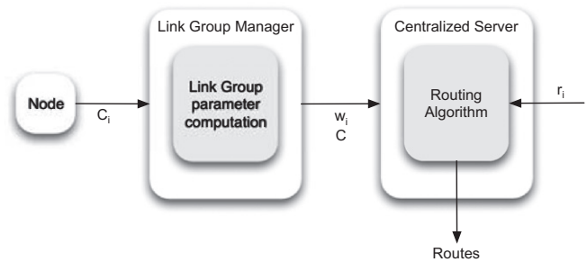
Fig. 13. Protocol operation.
