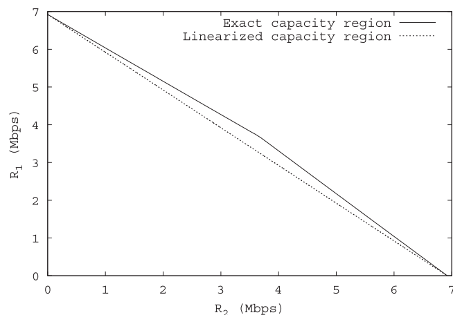
Fig. 4. Two nodes, homogeneous rates, 11 Mbps.
