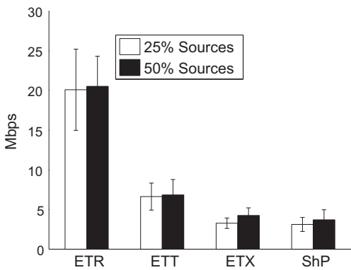
Fig. 14. Routing performance, 10% GW nodes.
