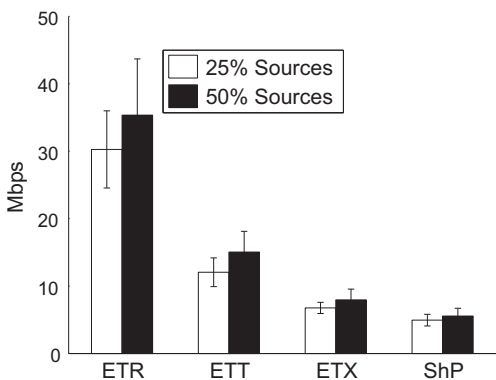
Fig. 15. Routing performance, 25% GW nodes.
