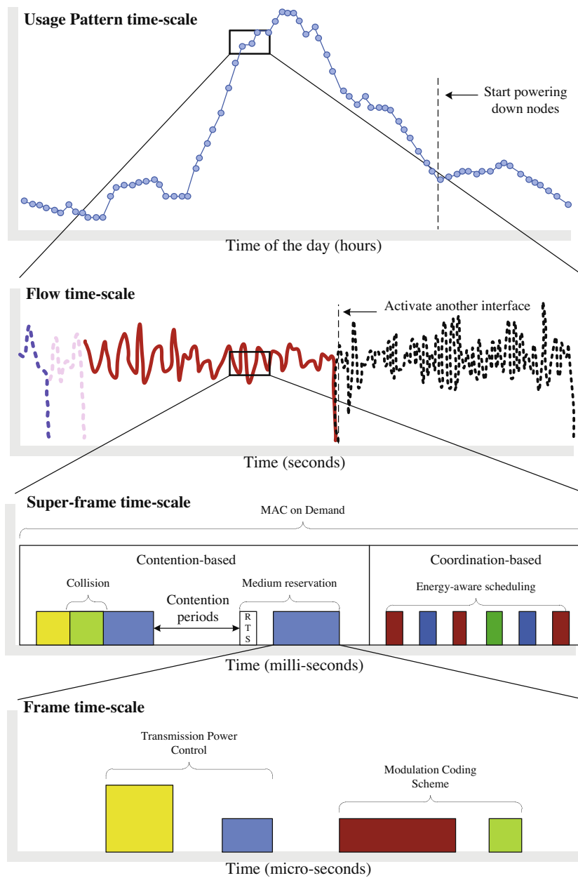
Fig. 1. Operational time-scales of the energy-saving algorithms.
