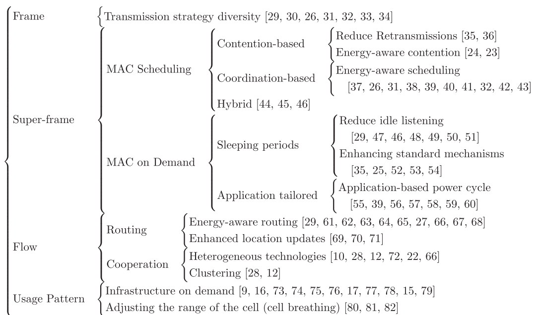
Fig. 2. Time-scale classification of energy efficient mechanisms.
