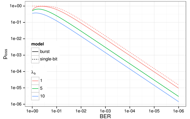
Figure 5: Frame loss probability given a BER level.
