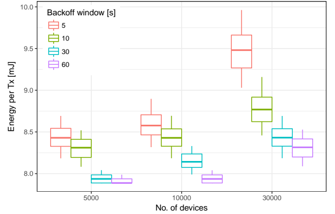
Fig. 4. Energy consumption per transmission attempt for different traffic models and number of devices.
