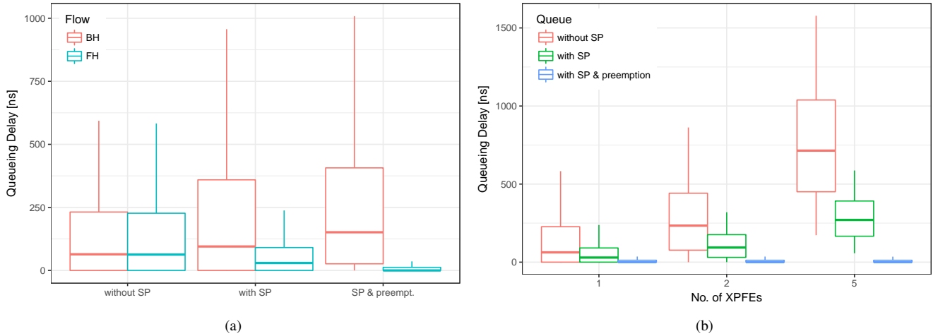
Fig. 2. Queueing delay experienced by FH and BH traffic under different QoS policies: a) FH/BH queueing delay comparison for a single XPFE; b) accumulated FH delay for several XPFEs. The whiskers represent the 5th and 95th percentiles.
