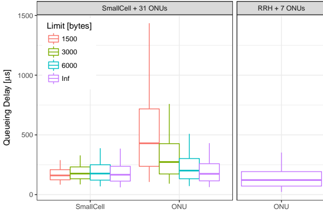
Fig. 3. Upstream delay for small cell and residential users sharing the upstream channel in a TDM-PON.
