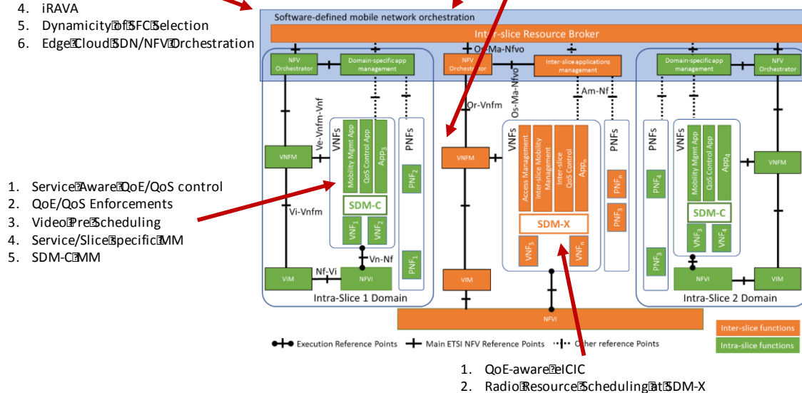
Figure-1-1: Mapping of the contributions of D5.2 to the WP5 functional architecture
