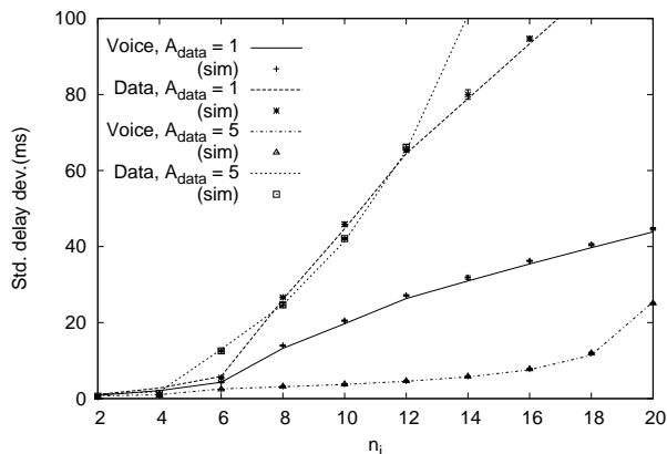
Fig. 10. Validation of the model of the standard deviation of the delay for a mixed scenario with voice and data stations and different AIFS configurations.
