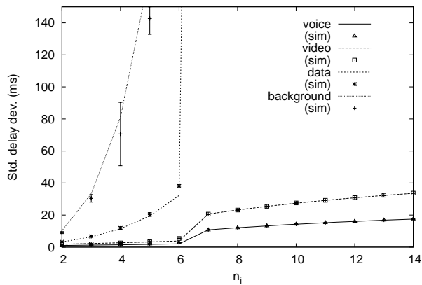
Fig. 13. Validation of the model for the standard deviation of the delay for a scenario with 4 ACs configured according to the standard recommended values.
