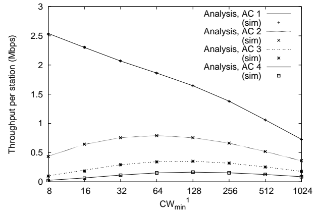
Fig. 5. Validation of the throughput model for a scenario with 4 ACs, each using a different AIFS and CW configuration.
