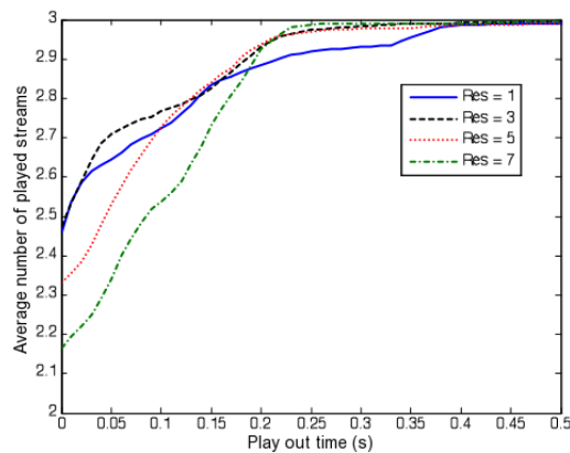
Figure 7. Average played streams for res=1,3,5,7
