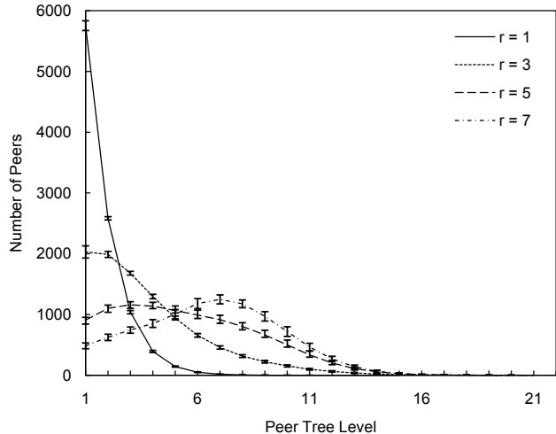
Figure 5. Number of peers at a certain level.
