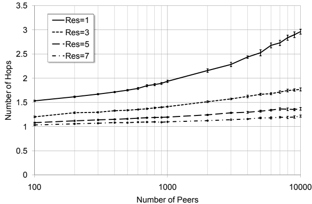
Figure 4. Average number of hops vs number of nodes.
