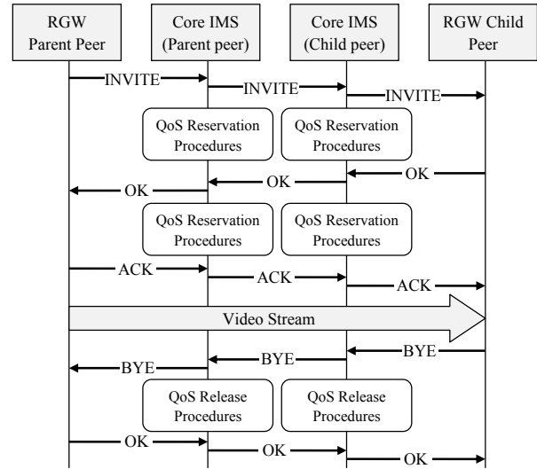
Figure 3. Session establishment and release scenario.
