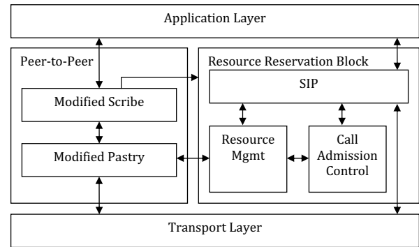
Figure 1. The protocol stack.
